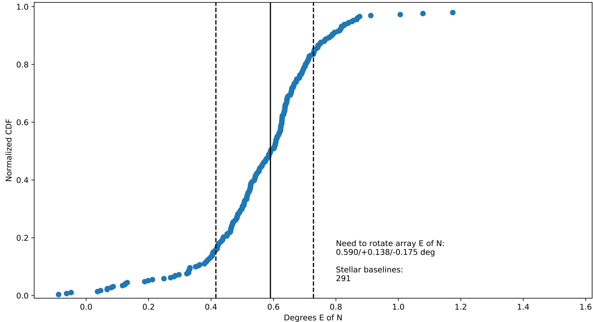
CDF of difference (E of N) between (RA, DEC) and (x, y) position angles on LMIRcam, Asterism UT 2018 Dec 24 (DX only)
