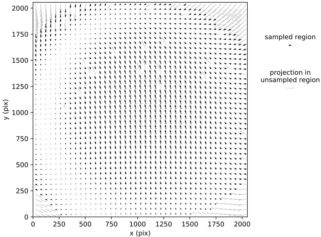
LMIRCam Distortion Correction Map (based on pinhole data taken Pinholes UT 2019 Jan 25 (SX only))
